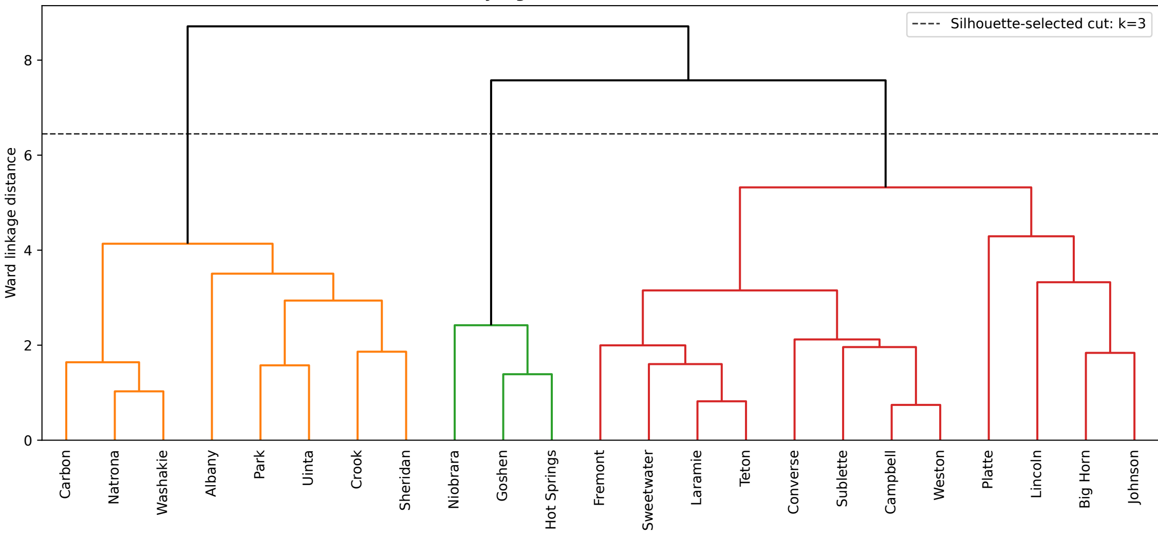
Ward Dendrogram — Simplified 6-Feature Space, 7-day Sakoe-Chiba Band Branch colors forced by highest silhouette score: k=3, silhouette=0.263
